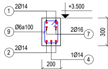
MC 8-8 2X1 (TL: 1/25)
