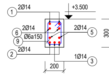
MC 4-4 2X1 (TL: 1/25)
