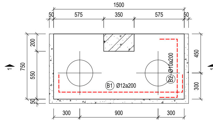
MÓNG M3a (SL=1)
